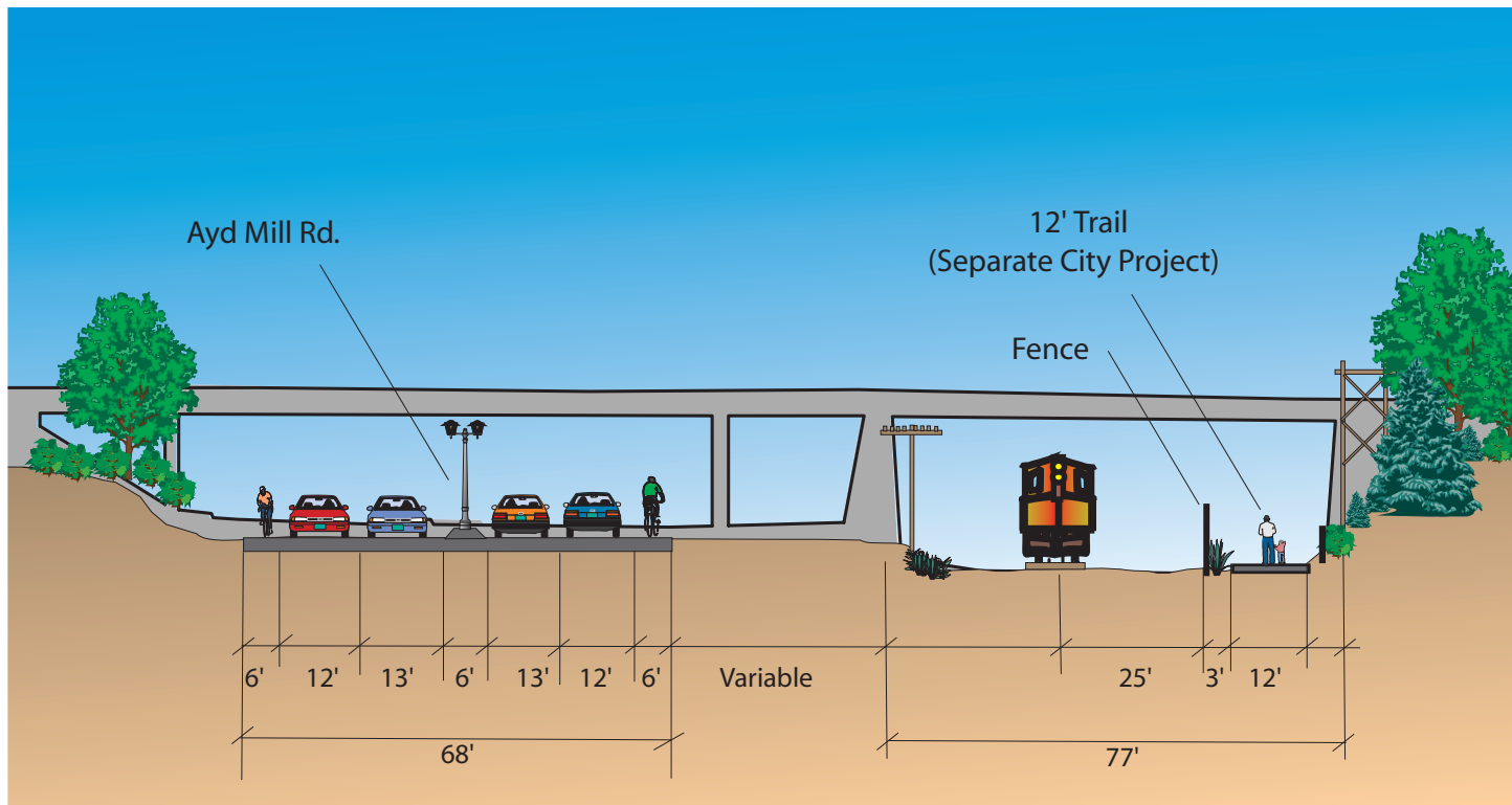
Ayd Mill Road Under St. Clair Avenue (Typical Section) Note: Bridge segments are similar for Grand Ave.
