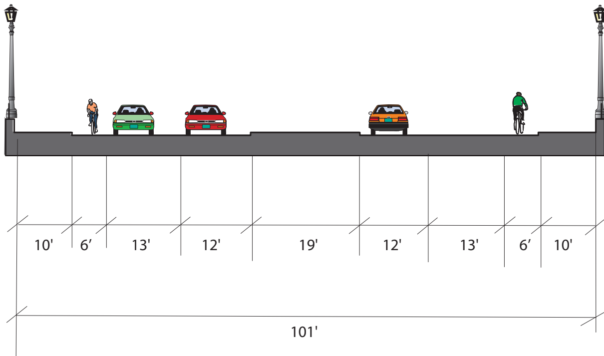
New Ayd Mill Road Over I-94 (Typical Section)
